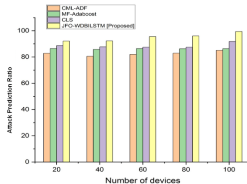
Fig. 3. Attack prediction ratio
