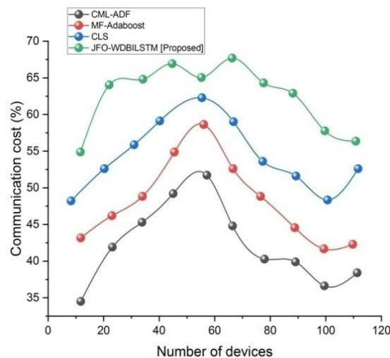
Fig. 6. Communication Cost Ratio
