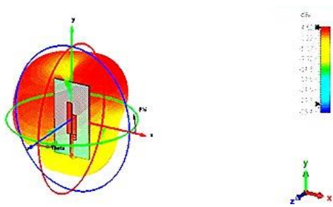
Fig. 7: The proposed antenna's far field plot (f=4.5 GHz)
