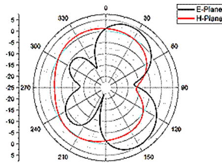
Fig.10. 4.5 GHz Frequency
