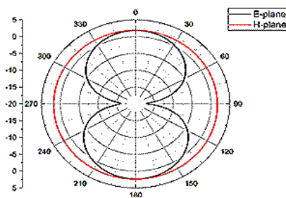
Fig.8. 1.8 GHz Frequency
