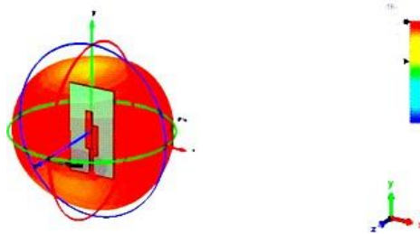
Fig. 6: The proposed antenna's far field plot (f=2.4 GHz)
