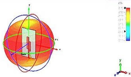
Fig. 5: The proposed antenna's far field plot (f=1.8 GHz)
