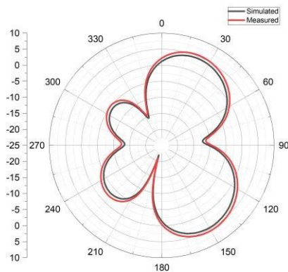
Fig 19. Result of E-plane. 4.5 GHz
