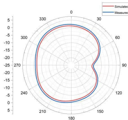
Fig.20 Result of H-plane. 4.5 GHz
