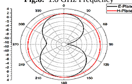
Fig.9. 2.4 GHz Frequency .
