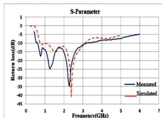
Fig. 14: Return loss of fabricated antenna measured using VNA
